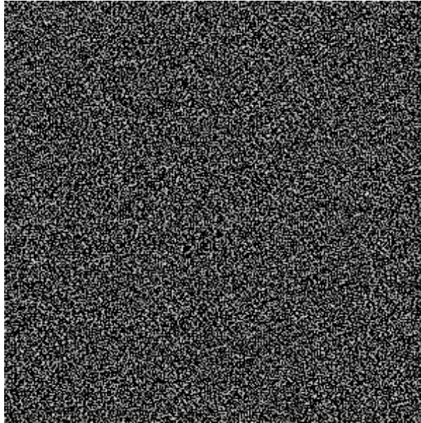
Figure 381: Example of Random Noise
